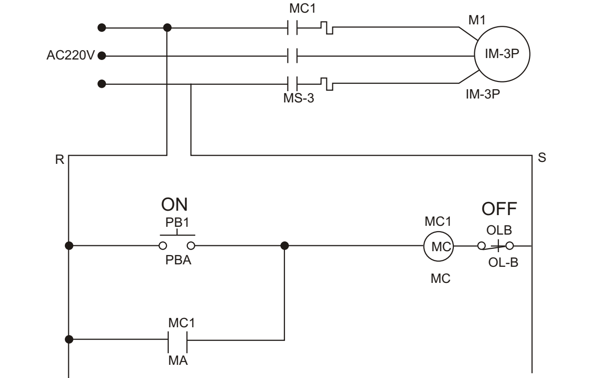
Circuit Diagram-3ph
