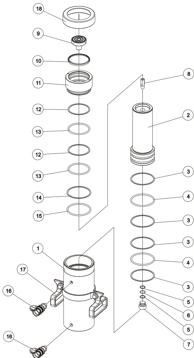
K1-Double-Acting, Stop ring, Plunger threads, Safety Assembly-plunger , Grooved saddle Cylinders(RSR-756)
