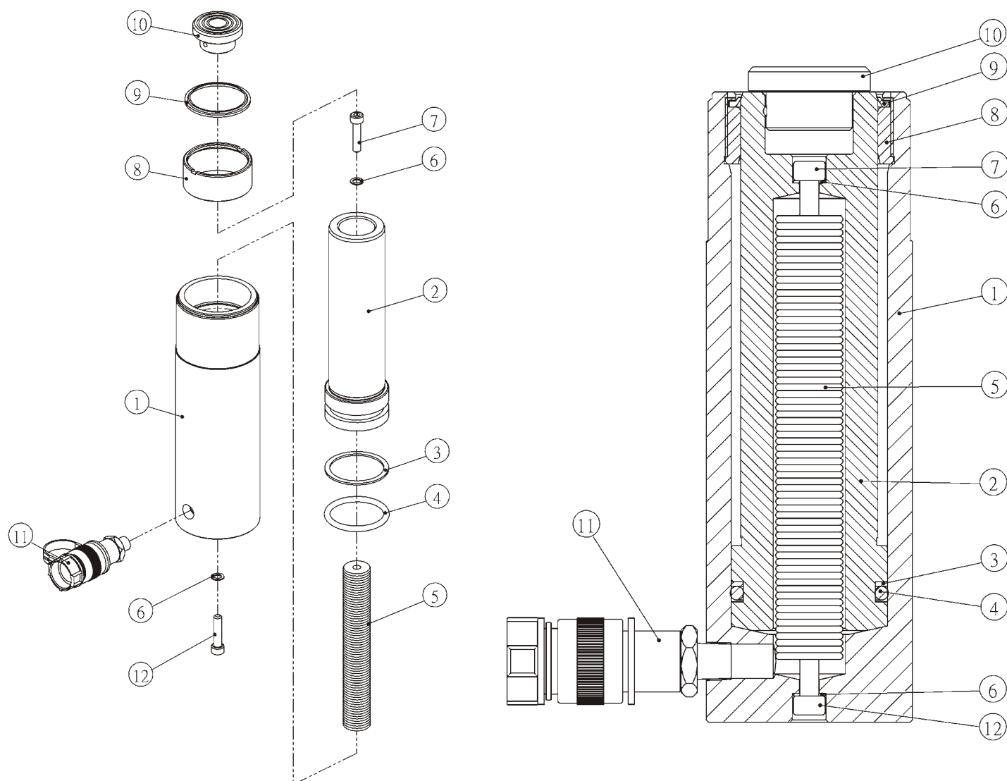
C-Single Acting,Stop ring,Plunger threads, Grooved(snap-in) saddle Cylinders (RSC-256)
