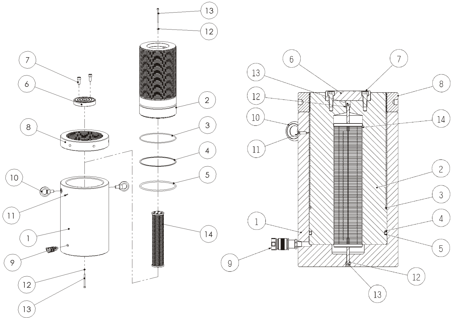
Q1-Single Acting,High Tonnage,Lock Nut Cylinders-Spring(CSLL-40012XF)
