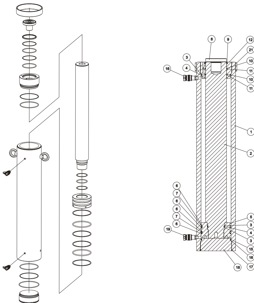
M-Double-Acting,Bace,Plunger inner threads,Stop ring, Grooved saddle Cylinders(RSR-40018)
