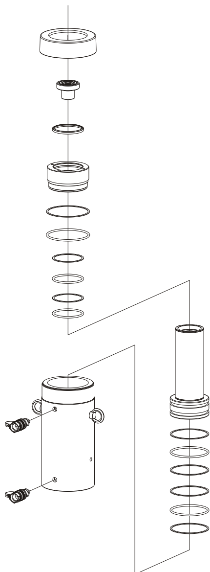
K-Double-Acting, Stop ring, Plunger threads, Safety Assembly- stop ring , Grooved saddle Cylinders (RSR-10013)
