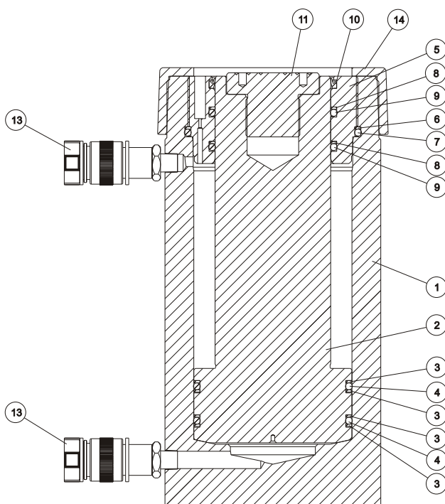
K-Double-Acting, Stop ring, Plunger threads, Safety Assembly- stop ring , Grooved saddle Cylinders (RSR-10013)
