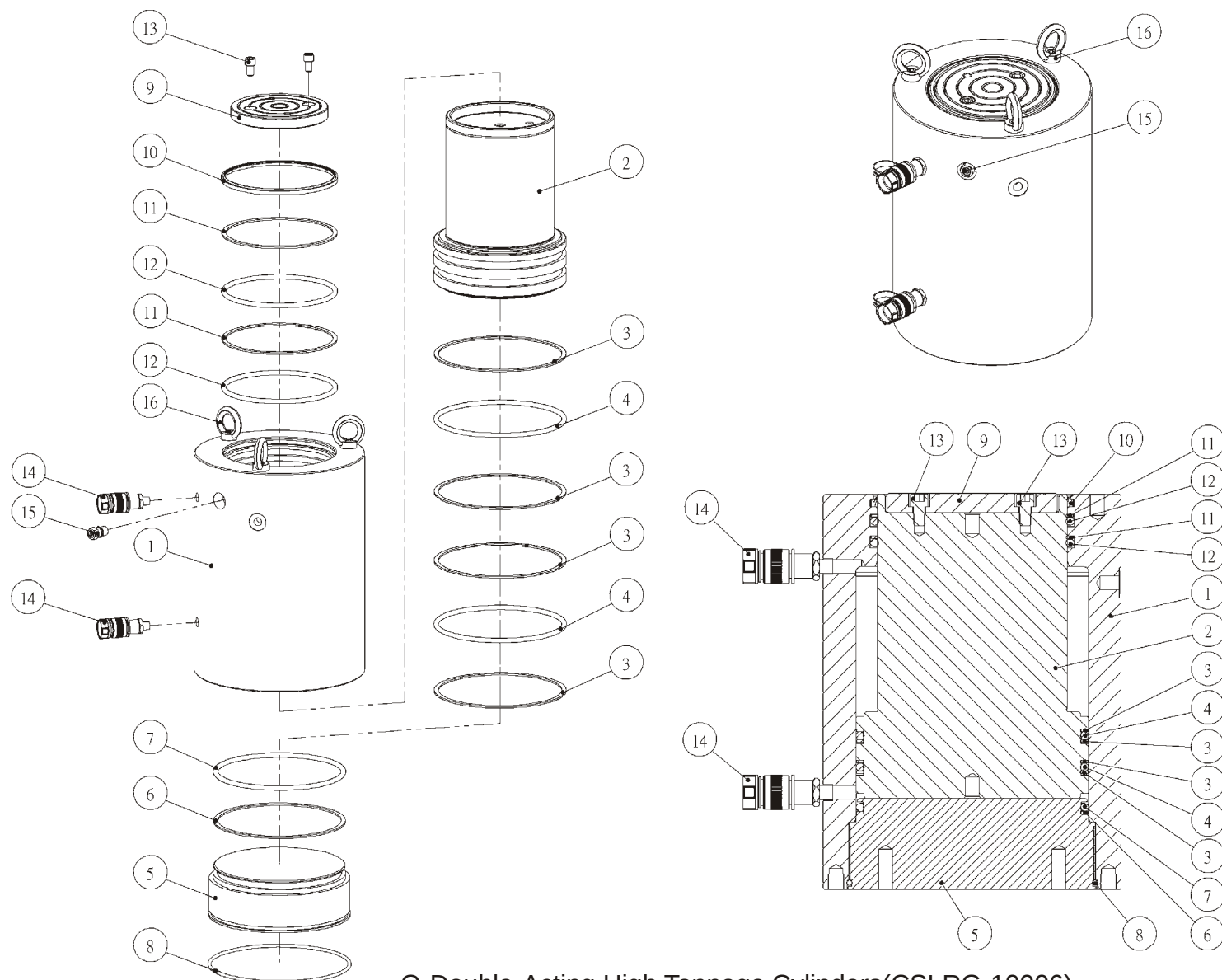
O-Double-Acting,High Tonnage Cylinders(CSLRG-10006)
