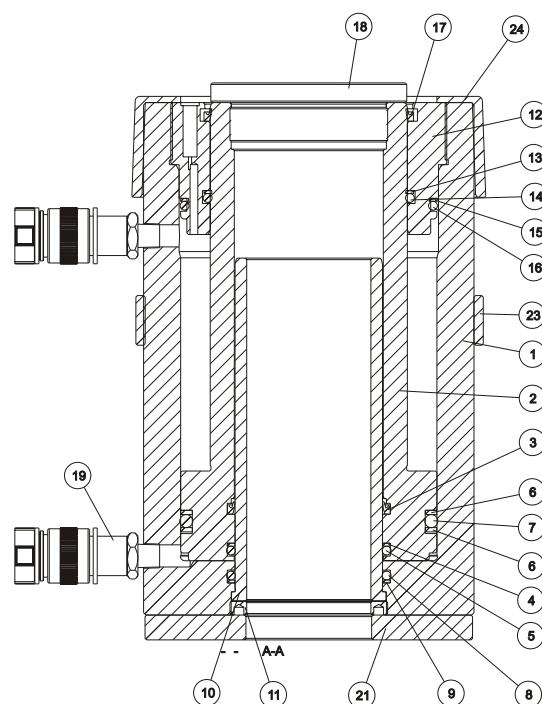
H1-Double-Acting,Hollow Plunger Cylinders(RSRH-603)
