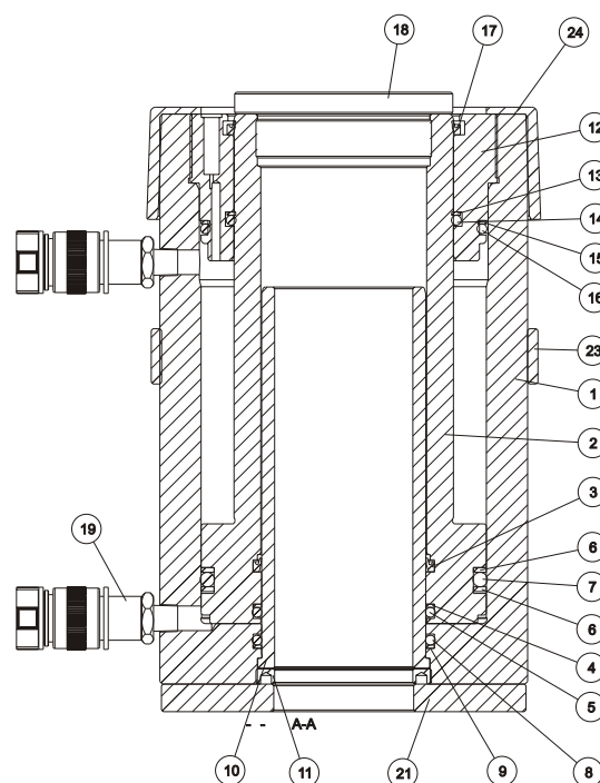
H1-Double-Acting,Hollow Plunger Cylinders(RSRH-6010)
